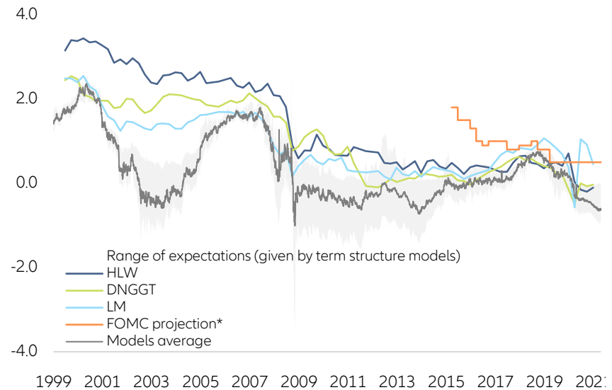
Figure 8 – Real equilibrium rate : macro models vs term structure models
