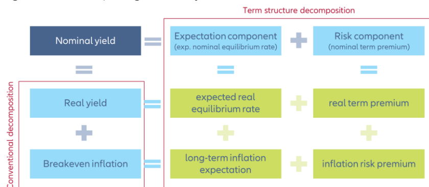
Figure 3 – Decomposing nominal yields
