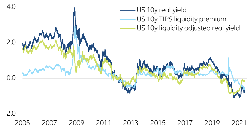
Figure 2 - Real yields are highly distorted by tight market conditions
